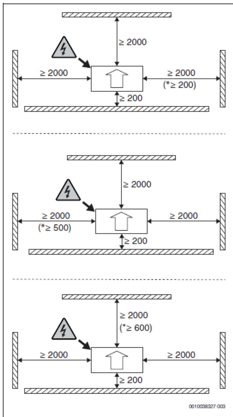
Fig. 12 Space between the heat pump and surrounding solid objects
